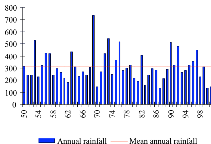
Fig. 82: Annual rain distribution in Kairouan (1950-2001)
