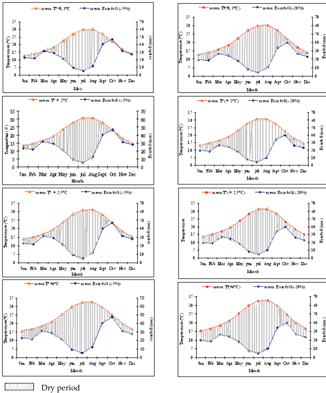
Fig.91: Gaussen Ombrothermic diagram in climate change conditions for Kairouan region.
