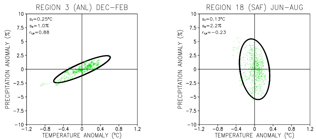
Fig. 4. The two-dimensional joint distribution of surface air temperature ( ^\circ\text{C} ) and normalized precipitation (%) anomalies in an unforced 1000 year simulation performed with CGCM2 for December-February over Antarctic land areas (Reg. 3, left panel) and for June-August over Southern Africa (Reg. 18, right panel). The regions are defined in Table 2. Small green dots depict the temperature and precipitation anomalies in individual overlapping 30 year periods. The thick black curve is the 95% contour ellipse of the two-dimensional normal distribution adjusted to the anomaly data. On the top-left corner of the panel are shown the parameters defining this normal distribution: standard deviations of the temperature and precipitation and their correlation.
