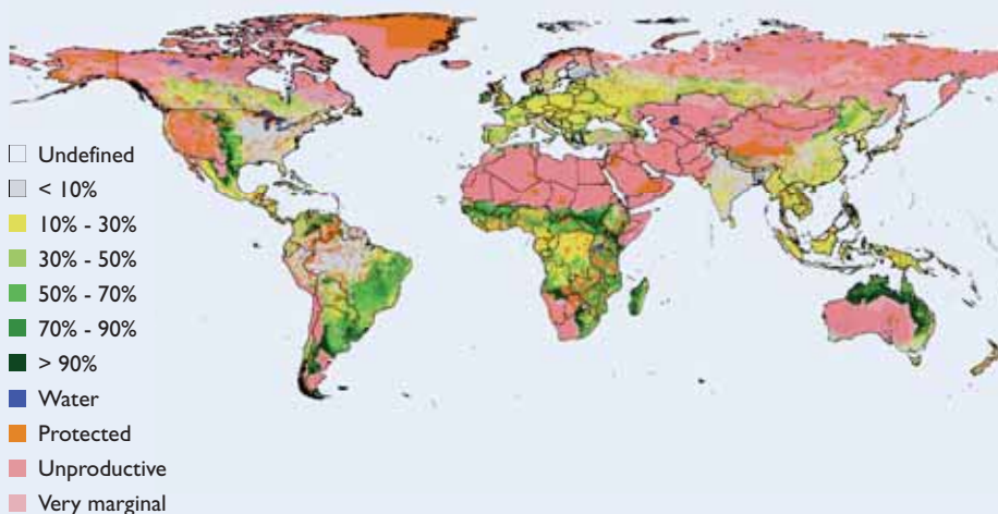
Spatial distribution and share of land by 5' latitude/longitude grid cell currently classified as unprotected grassland and woodland potentially useable for rain-fed ligno-cellulosic biofuels feedstock production
